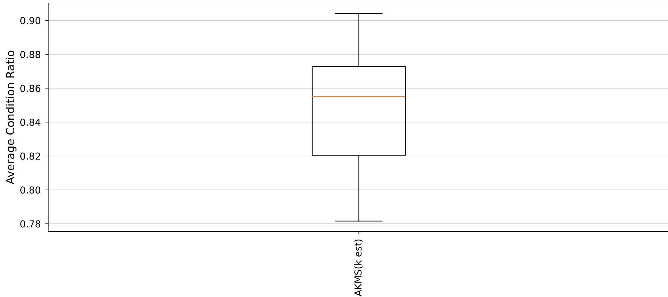
YARA Rules Average Condition Ratio Distribution (Cluster0_Size134 dataset)
